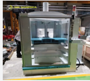
Customized Hydraulic Press
